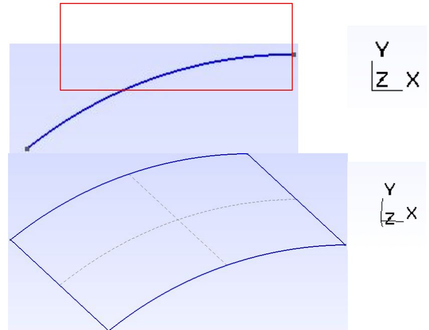
Exactly curvature surface 2
