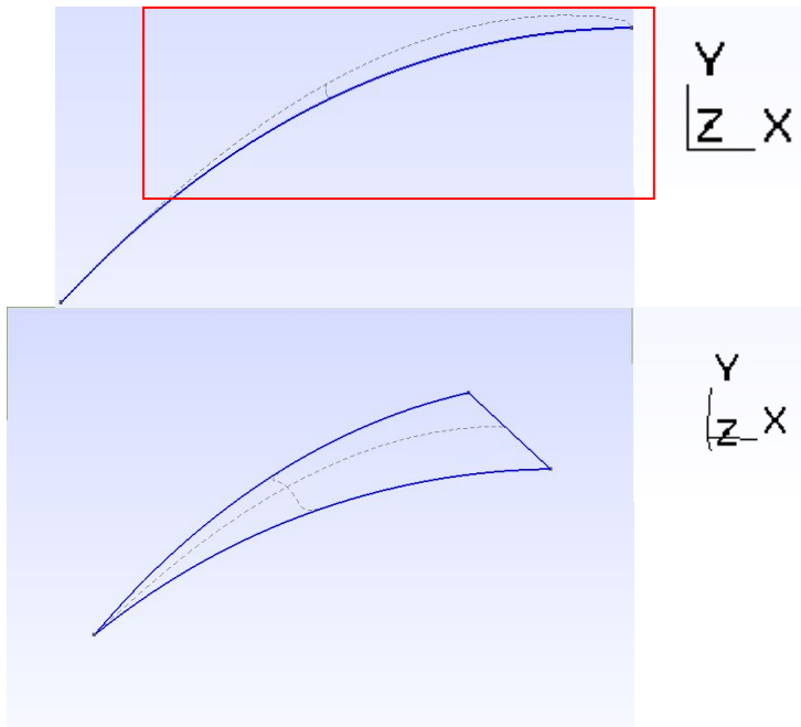
Error curvature surface 1
