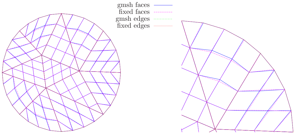
Figure 1: Curved 2D mesh (triangles): comparison of gmsh natives and fixed nodes.
