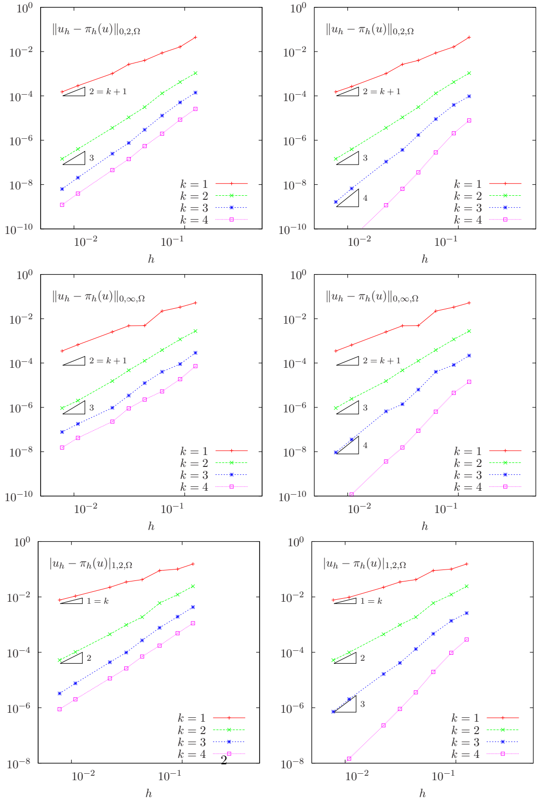
Figure 2: Curved 2D mesh (triangle): error analysis in L^2 , L^\infty and H^1 norms. Left: native gmsh ; right: fixed nodes.
